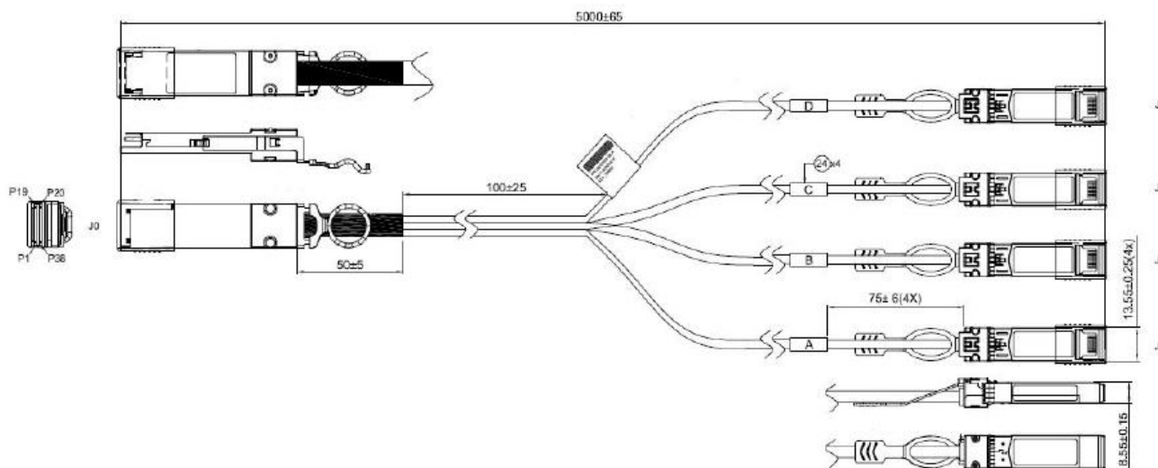
Mechanical Drawing
